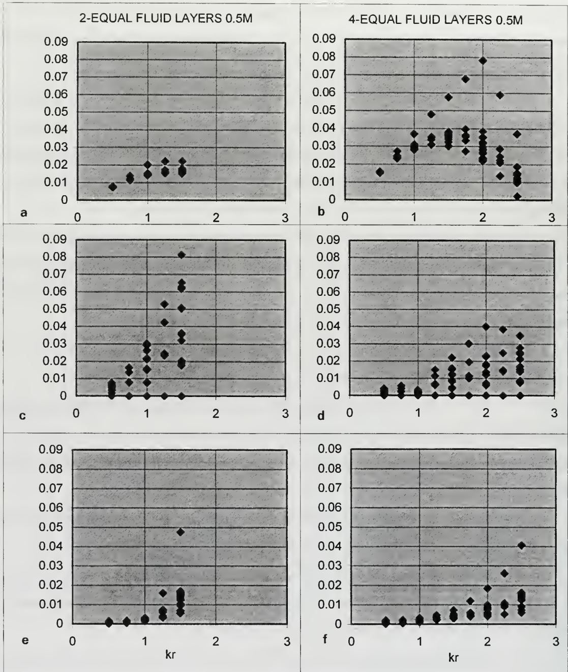
Figure 12. Normalized scattered pressure deviation computed by ATILA versus kr . From top to bottom monopolar (a,b), dipolar (c,d) and quadrupolar (e,f) incident field; on the left: radiation boundary at kR = 1.5 ; on the right: radiation boundary at kR = 2.5 ; scatterer radius a and element size L satisfy: ka = 0.5 and kL = 0.5 for all cases.
